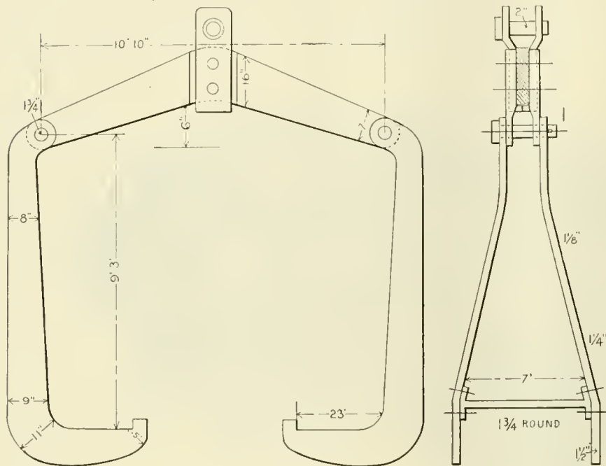
SLING YOKE FOR LIFTING TENDERS.
